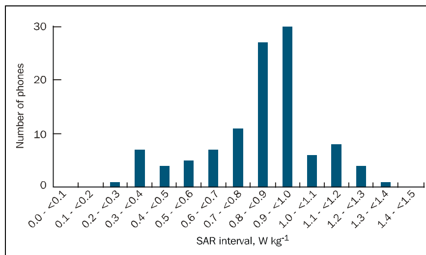
FIGURE 2.5 Distribution of SARs produced by 111 mobile phone handsets, as indicated by their manufacturers in June 2003
