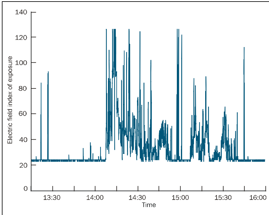
FIGURE 2.7 Electric field trace acquired from a body-mounted personal exposure meter worn by a worker at a VHF broadcast site
