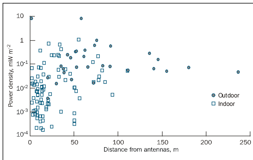
FIGURE 2.9 Total power density from local base stations
